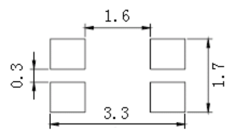
Recommended Soldering Pattern (Units : mm)
